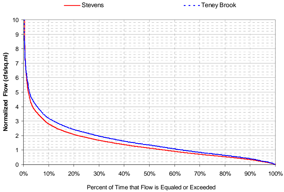
Figure 5. High flow portion of the flow duration curves for Stevens Brook and attainment stream.
