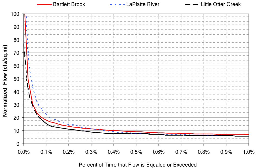
Figure 5. High flow portion of the flow duration curves for Bartlett Brook and attainment streams.
