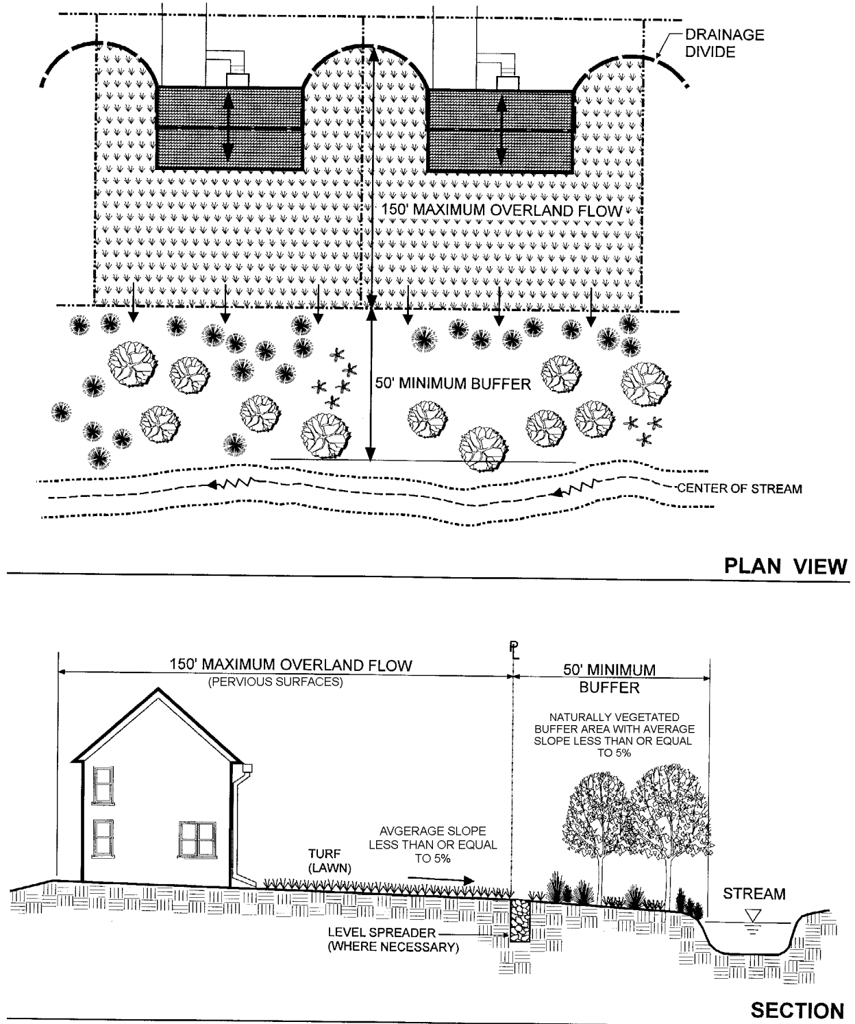
Figure 3.3 Example of Stream Buffer Credit Option
