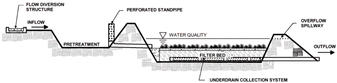
PROFILE
