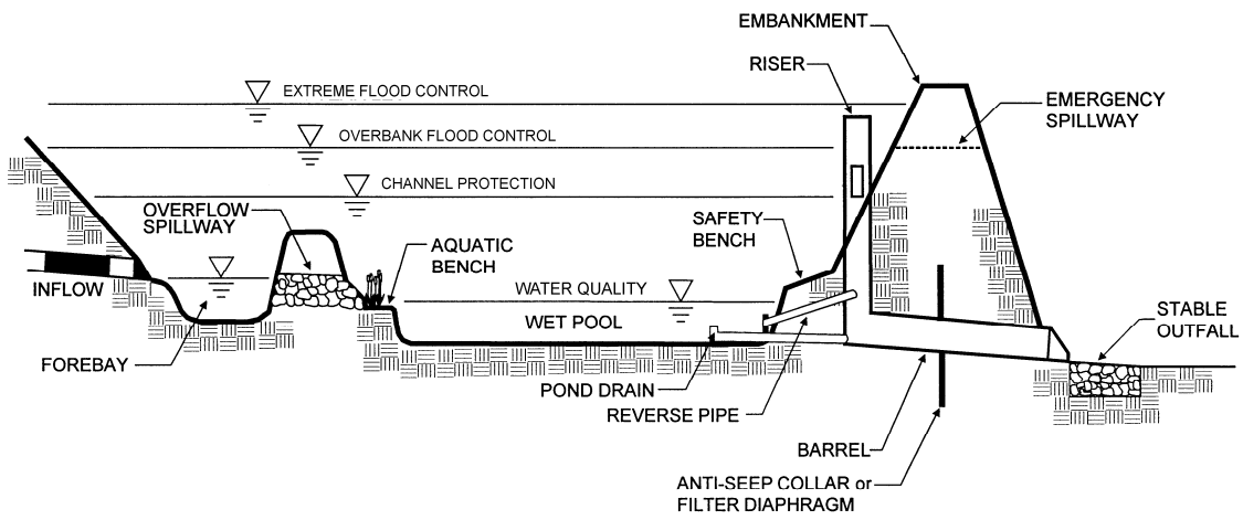
PROFILE
