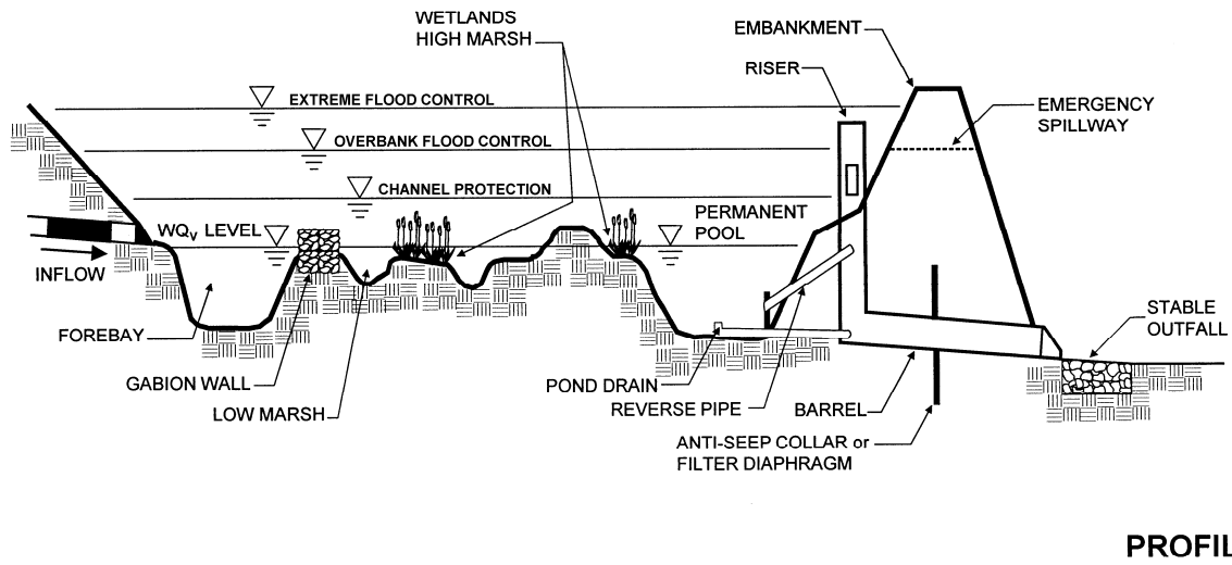
Figure 2.7 Example of Shallow Wetland (W-1)
