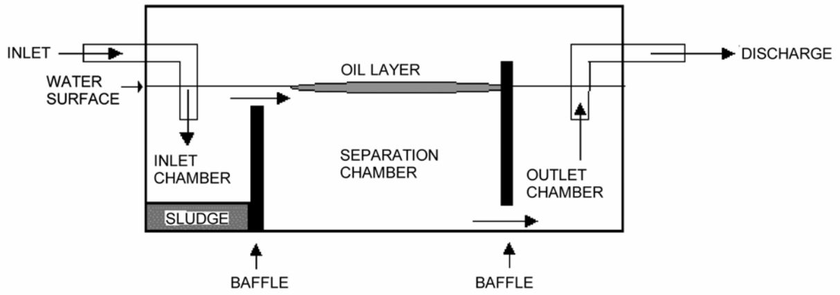
Figure 2.25 Example of Oil and Grit Separators (LA-4)
