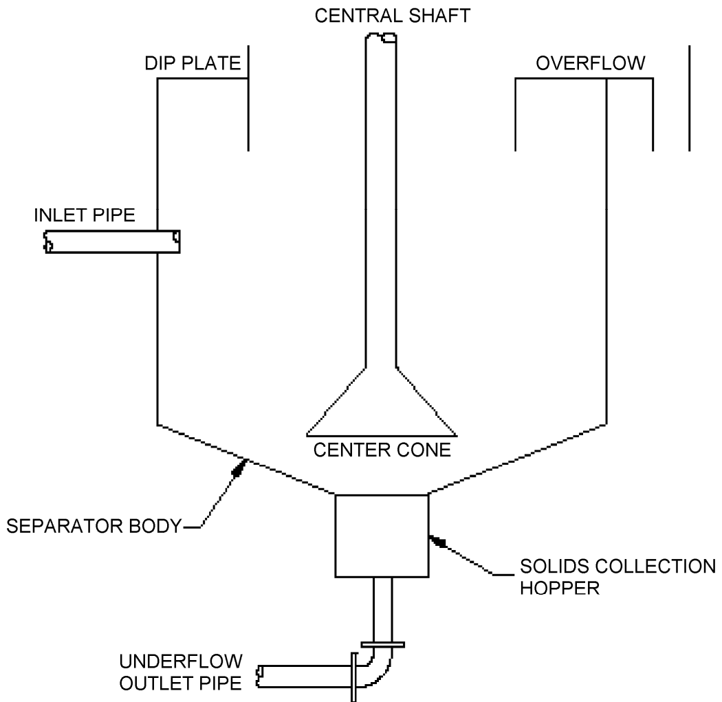
Figure 2.24 Example of Hydrodynamic Device (LA-3)
