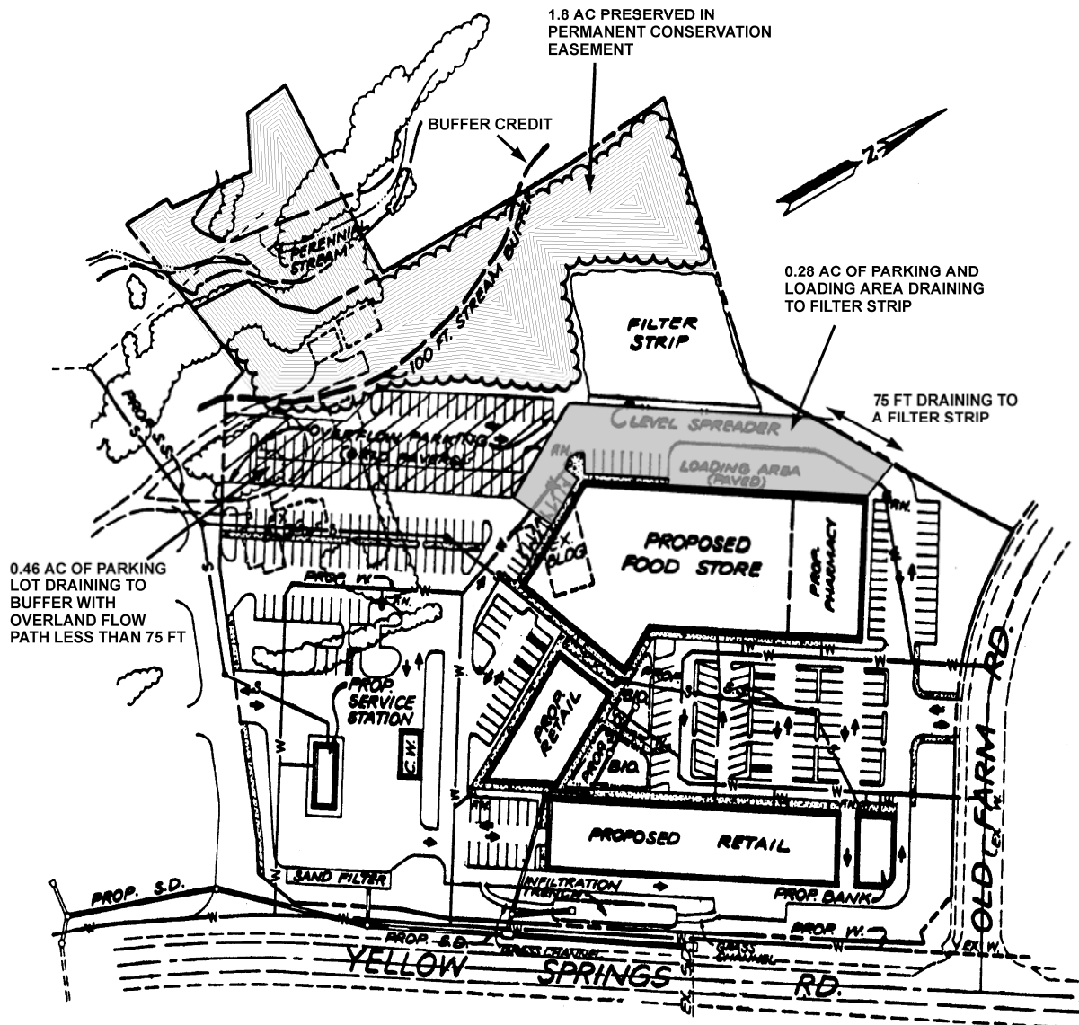
Figure 3.7 Example of Modified Retail Site Design
