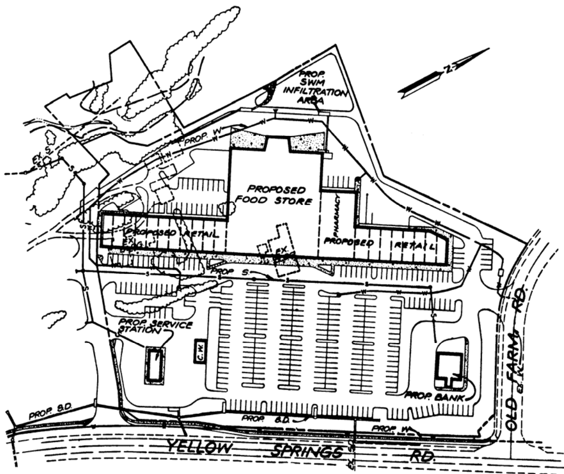
Figure 3.6 Example of Conventional Retail Site Design
