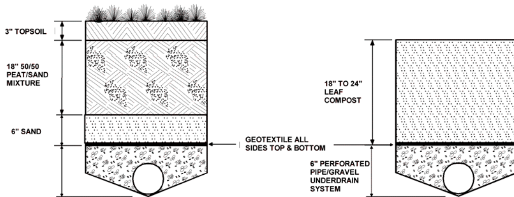
TYPICAL SECTIONS
