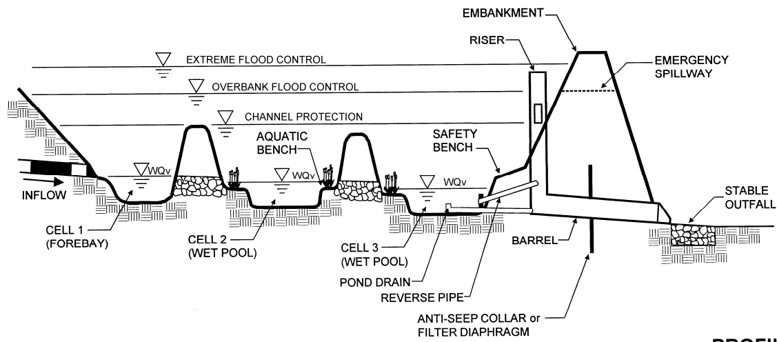
PROFILE
