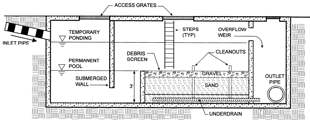
PROFILE
