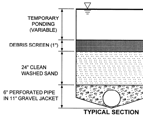
Figure 2.15 Example of Underground Sand Filter (F-2)
