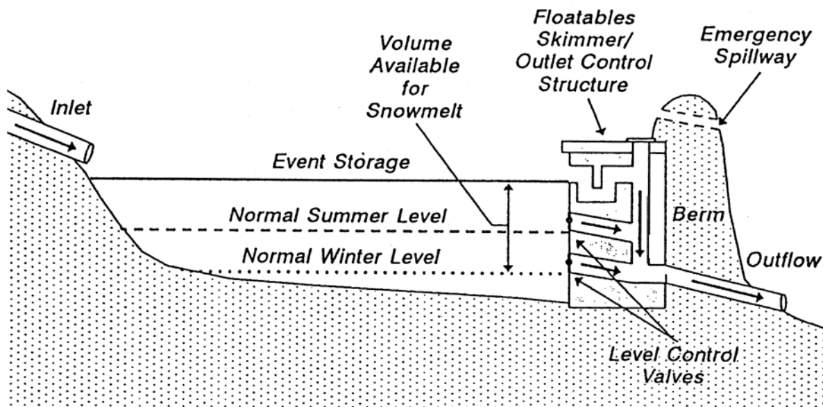
Figure 2.6 Seasonal Operation Pond (Source: Oberts, 1994)
