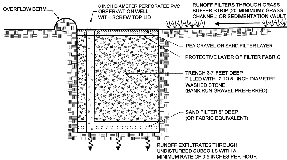
Figure 2.11 Example of Infiltration Trench (I-1)
