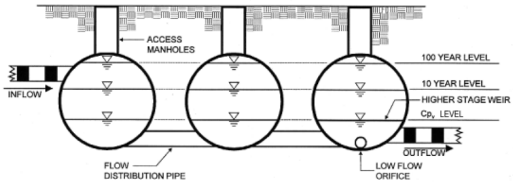
TYPICAL SECTION
