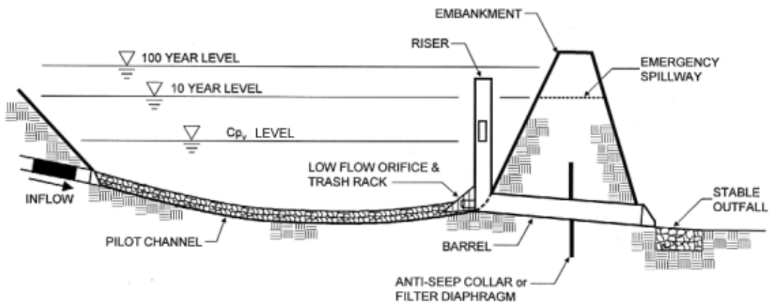
PROFILE
