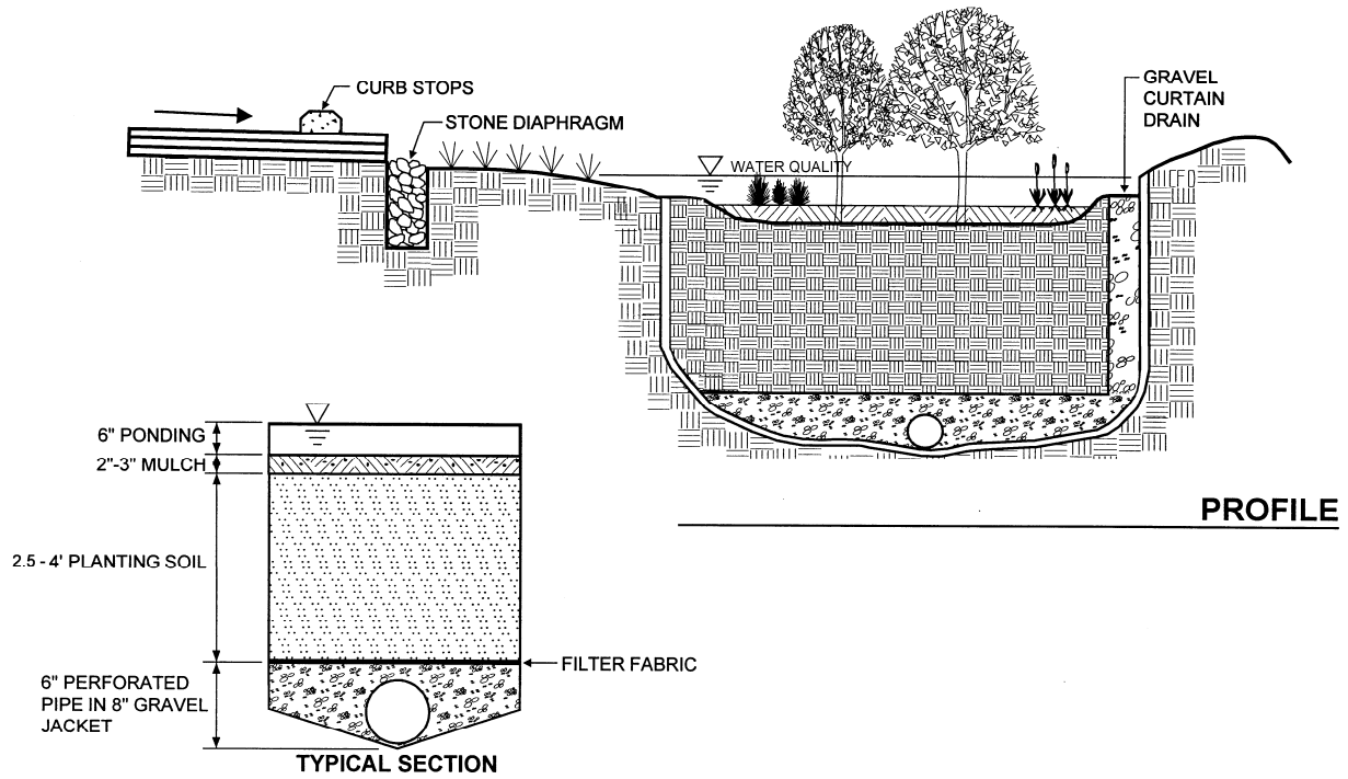
Figure 2.18 Example of Bioretention (F-5)
