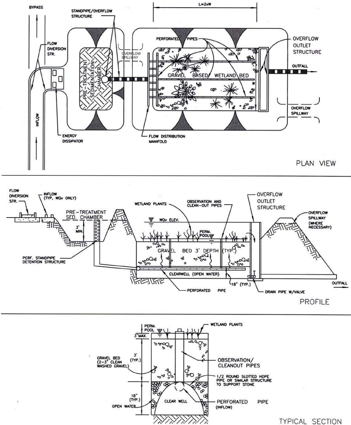
Figure 2.10 Example of Gravel Wetland (W-4)
