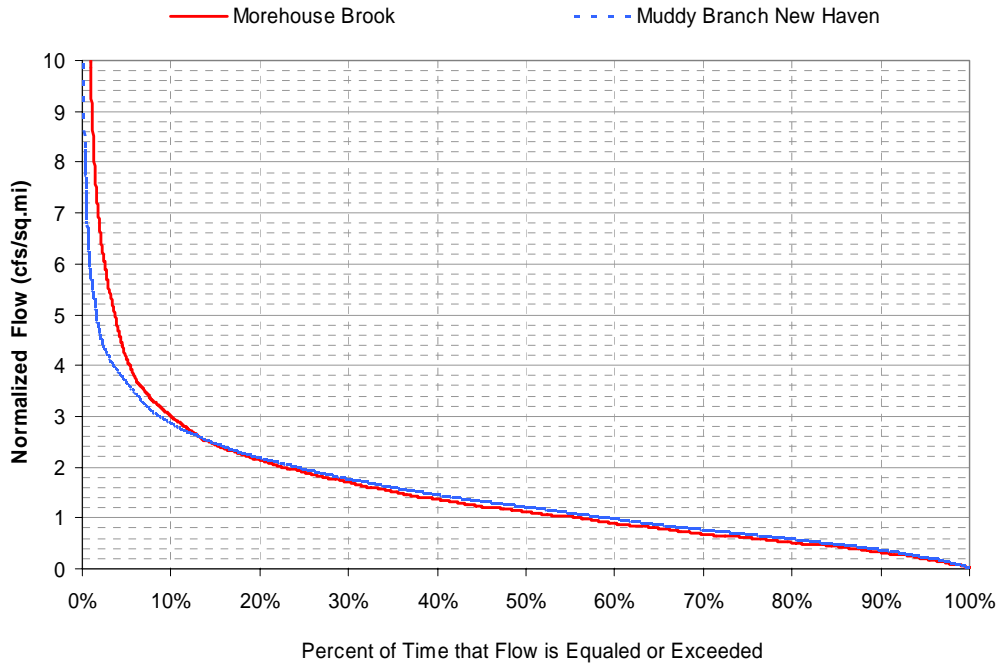
Figure 5. High flow portion of the flow duration curves for Morehouse Brook and attainment stream.
