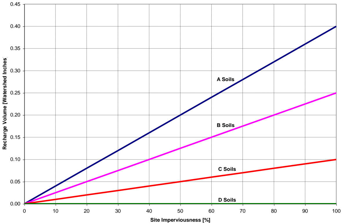
Figure 1.2 Relationship Between Recharge Requirement and Site Impervious Cover
