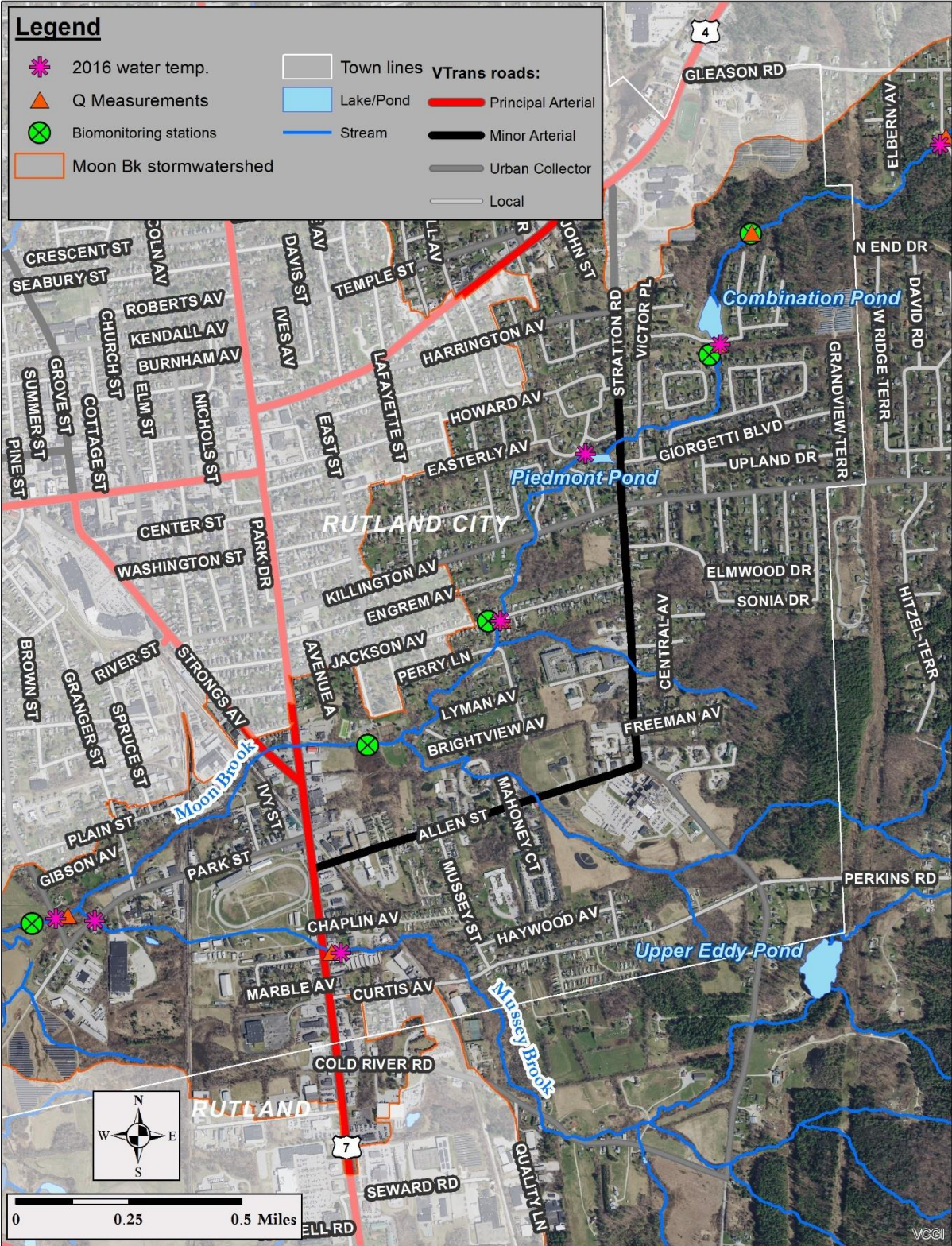
Figure 2. Area of interest in the Mussey Brook watershed.
