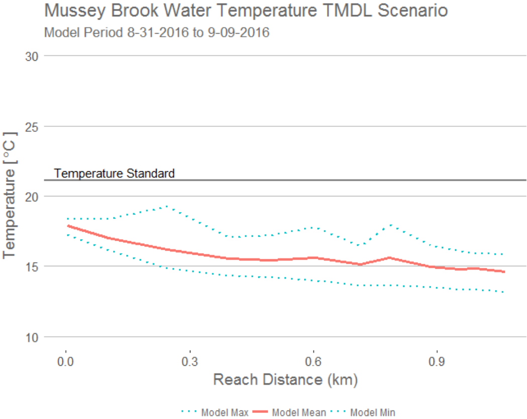
Figure 14. Predicted temperatures after applying the loading capacity scenario under critical conditions. The 0.0 km distance represents the uppermost stream temperature monitoring station (Section 5.2.1). Distances are measured from that point downstream.
