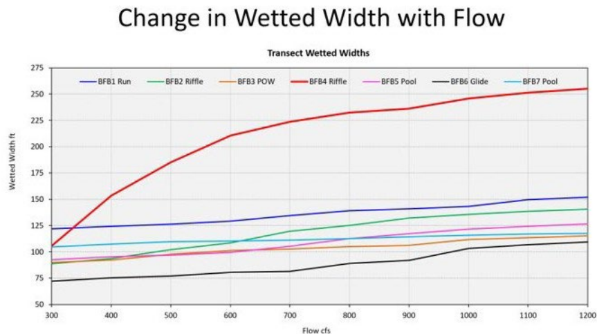
Figure 2. The graph shows the increase in wetted width with increase in flow (cfs) for all the transect measured as part of the Bellows Falls bypass flow habitat study. Transect 4 (red) wetted width increases at a relatively faster rate than the other transects in the study
