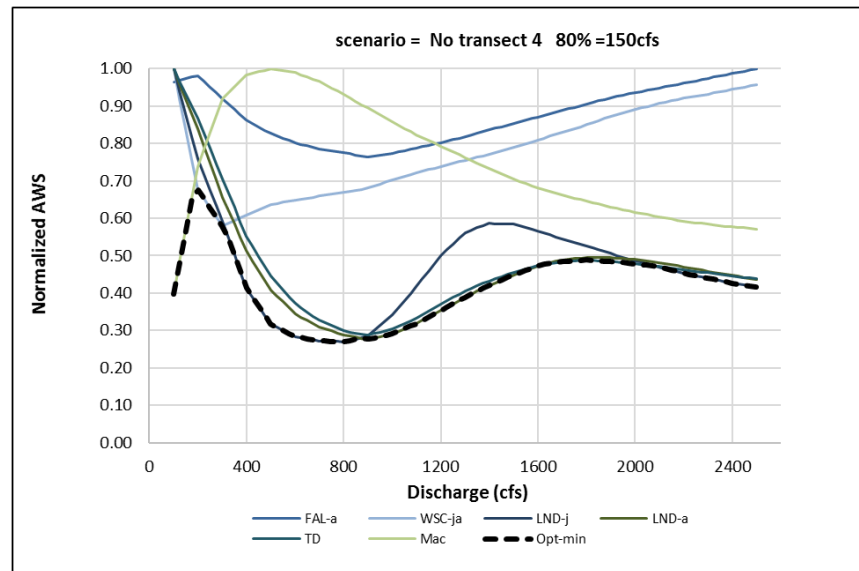
Figure 4. The relationship between flow and habitat (area weighted suitability, AWS) for target species and life stages for the Bellows Falls bypass reach of the Connecticut River below the Bellows Falls Hydroelectric Project with transect four omitted from the analysis. Species included are Fallfish adult (FAL-a), White Sucker juveniles and adults (WSC-ja), Longnose Dace juveniles (LND-j), Longnose Dace adults (LND-a), Tessellated Darter (TD), and macroinvertebrates (Mac). The dash line is the optimization minimum.
