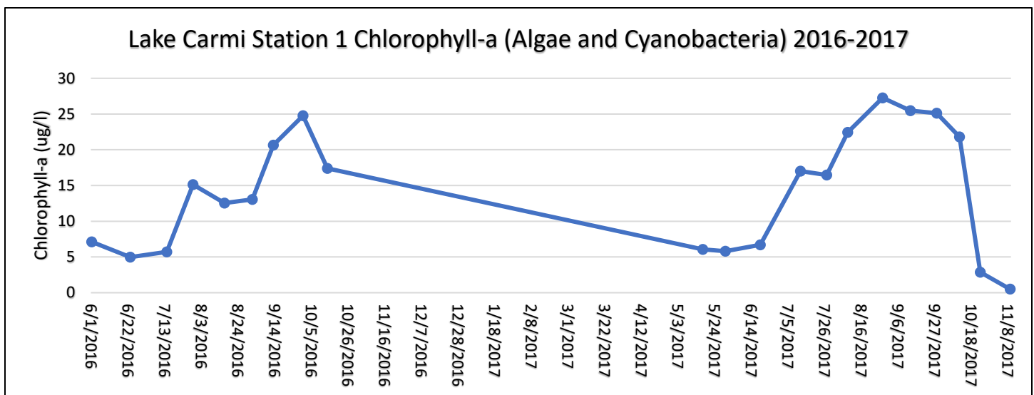
Figure 1. Chlorophyll-a measured as a proxy for algae/cyanobacteria concentration (intense prolonged blooms in summer/fall 2017).
