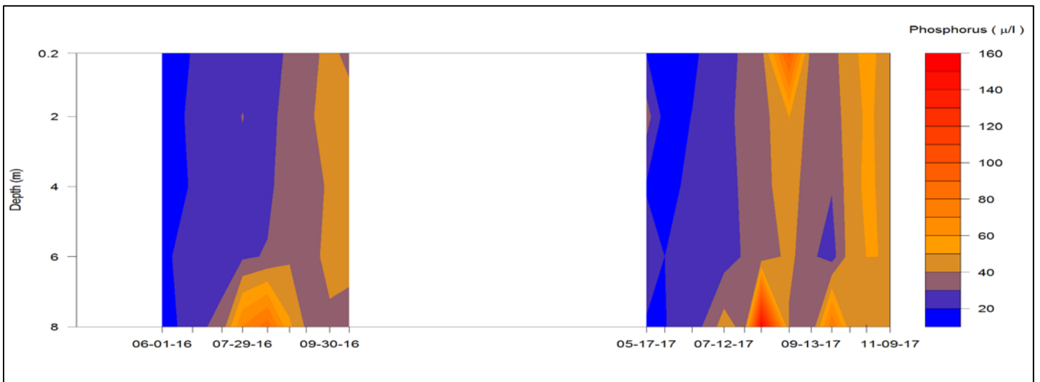
Figure 6. Lake Carmi Station 1 Total Phosphorus Vertical Profiles 2016-2017: Note that internal loading occurred twice in 2017.
