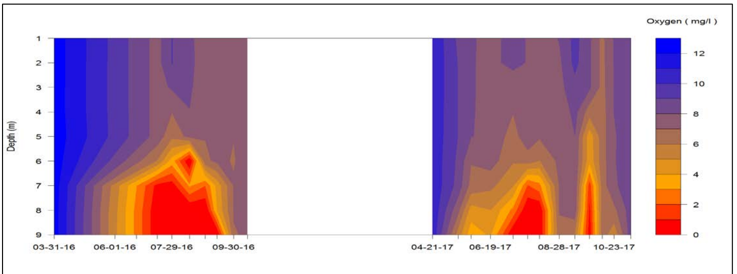
Figure 5. Lake Carmi Station 1 Dissolved Oxygen Vertical Profiles 2016-2017: Note that oxygen depletion occurred twice in 2017.
