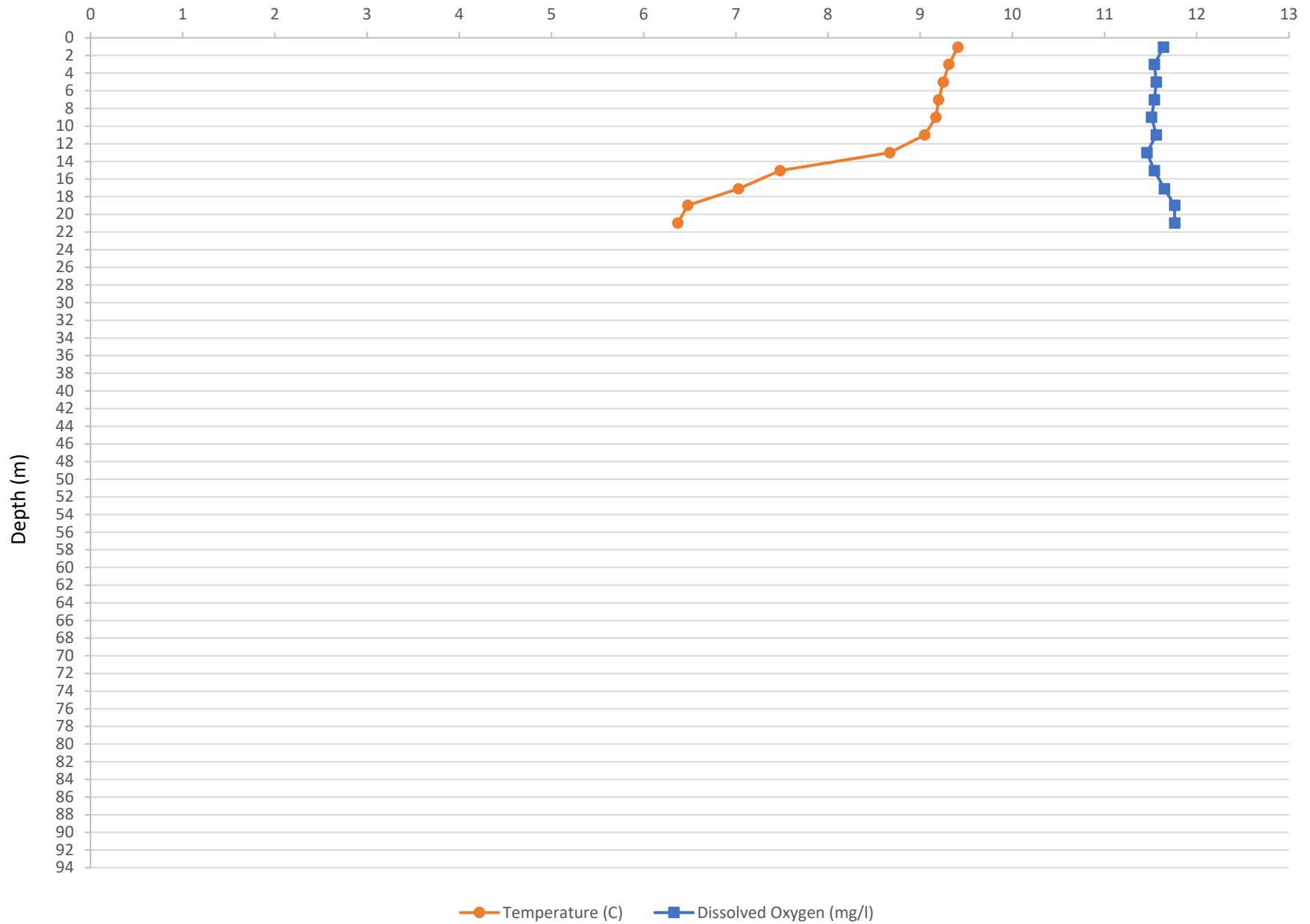
Lake Willoughby Station 1 Temperature and Dissolved Oxygen Profiles on 6/6/2017
