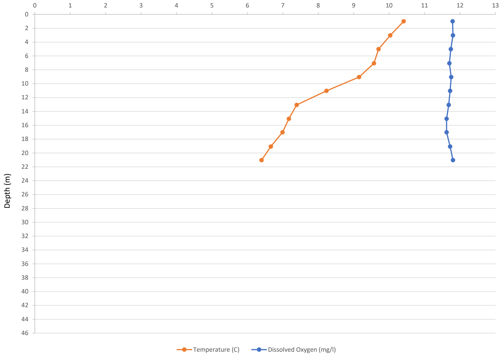
Lake Willoughby Station 2 Temperature and Dissolved Oxygen Profiles on 6/6/2017
