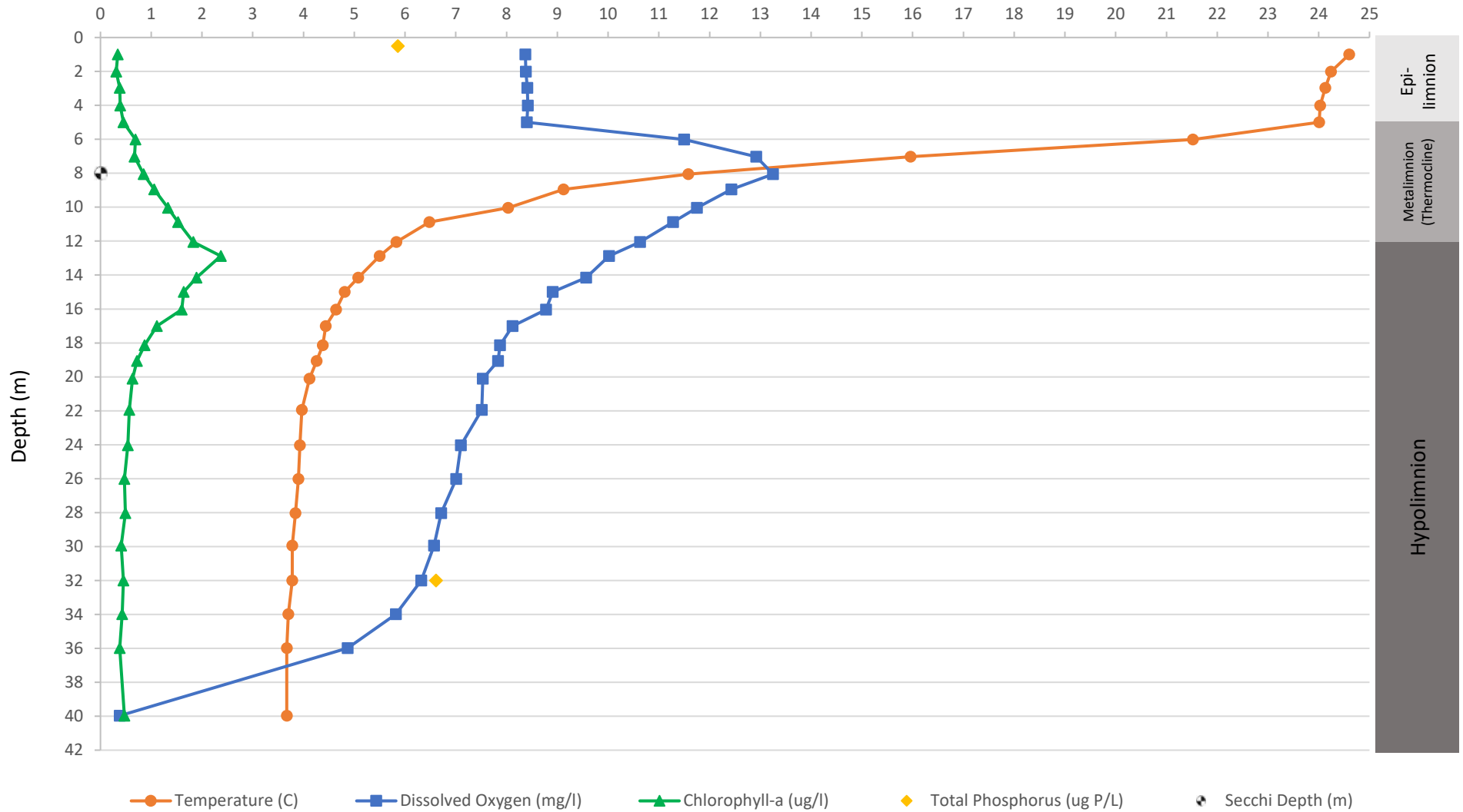
Shadow Lake (Glover) Station 1 Temperature, Dissolved Oxygen, Chlorophyll-a and Total Phosphorus Vertical Profiles on 8/13/2018
