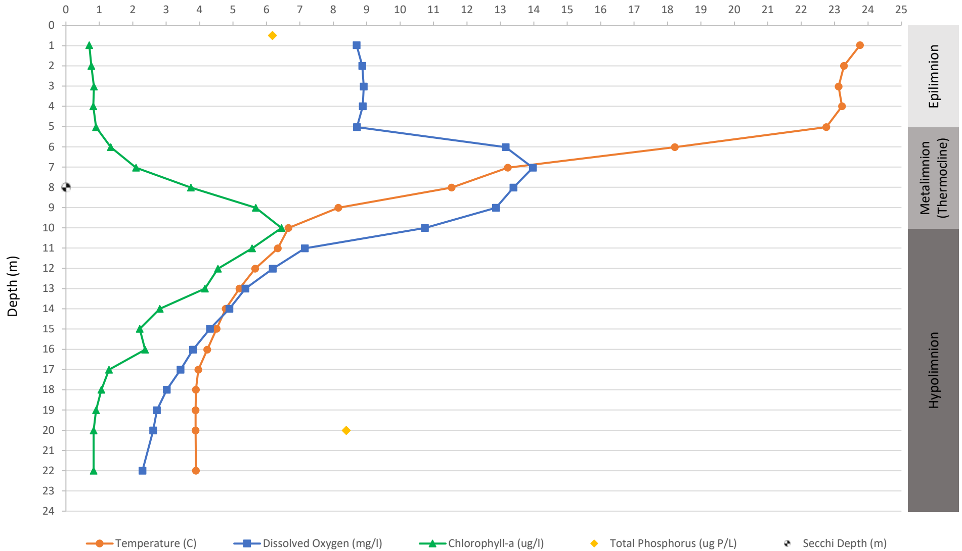
Nichols Pond Station 1 Temperature, Dissolved Oxygen, Chlorophyll-a and Total Phosphorus Vertical Profiles on 8/27/2018
