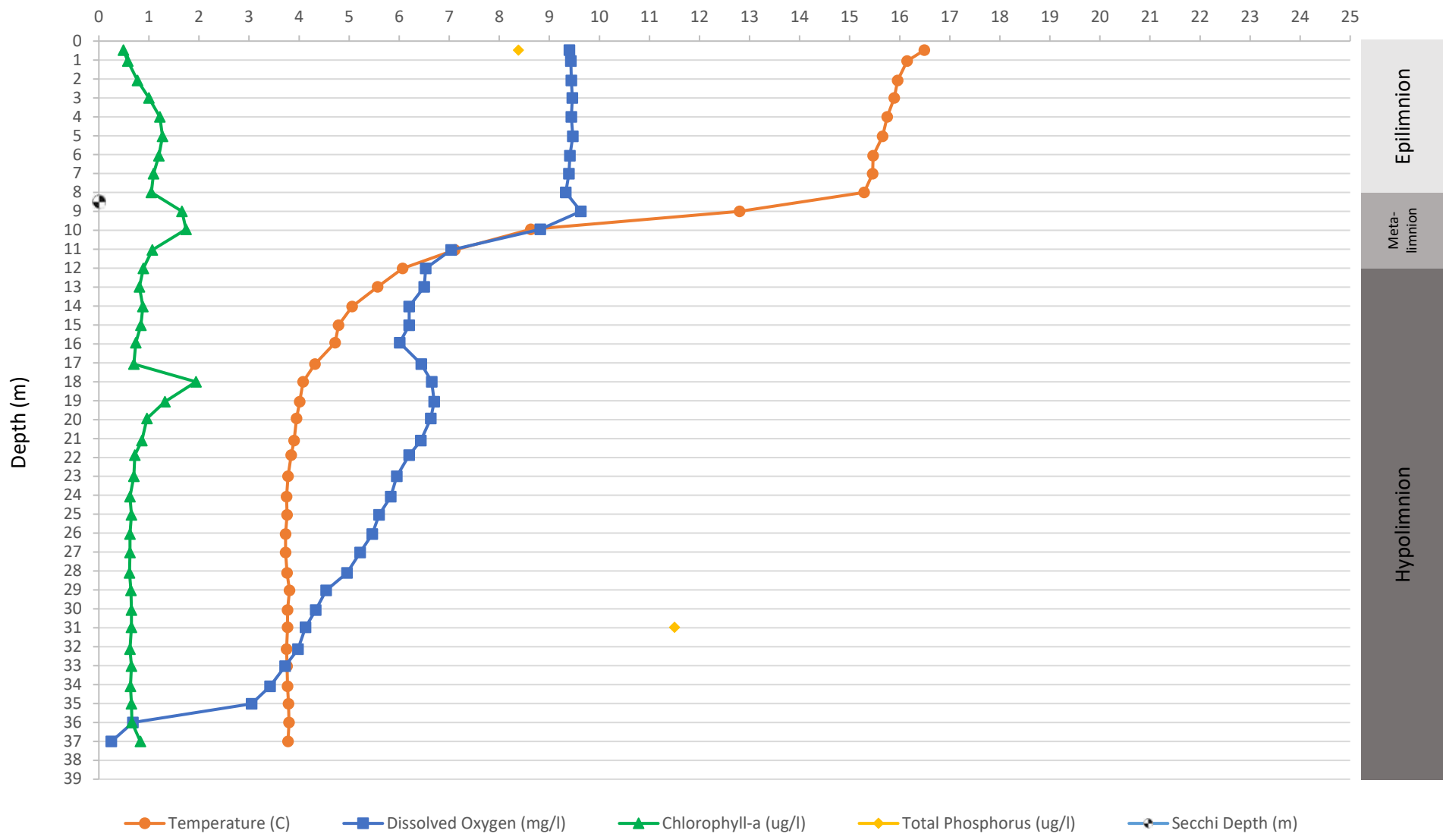
Harvey's Lake Station 1 Temperature, Dissolved Oxygen, Chlorophyll-a and Total Phosphorus Vertical Profiles on 10/10/2018
