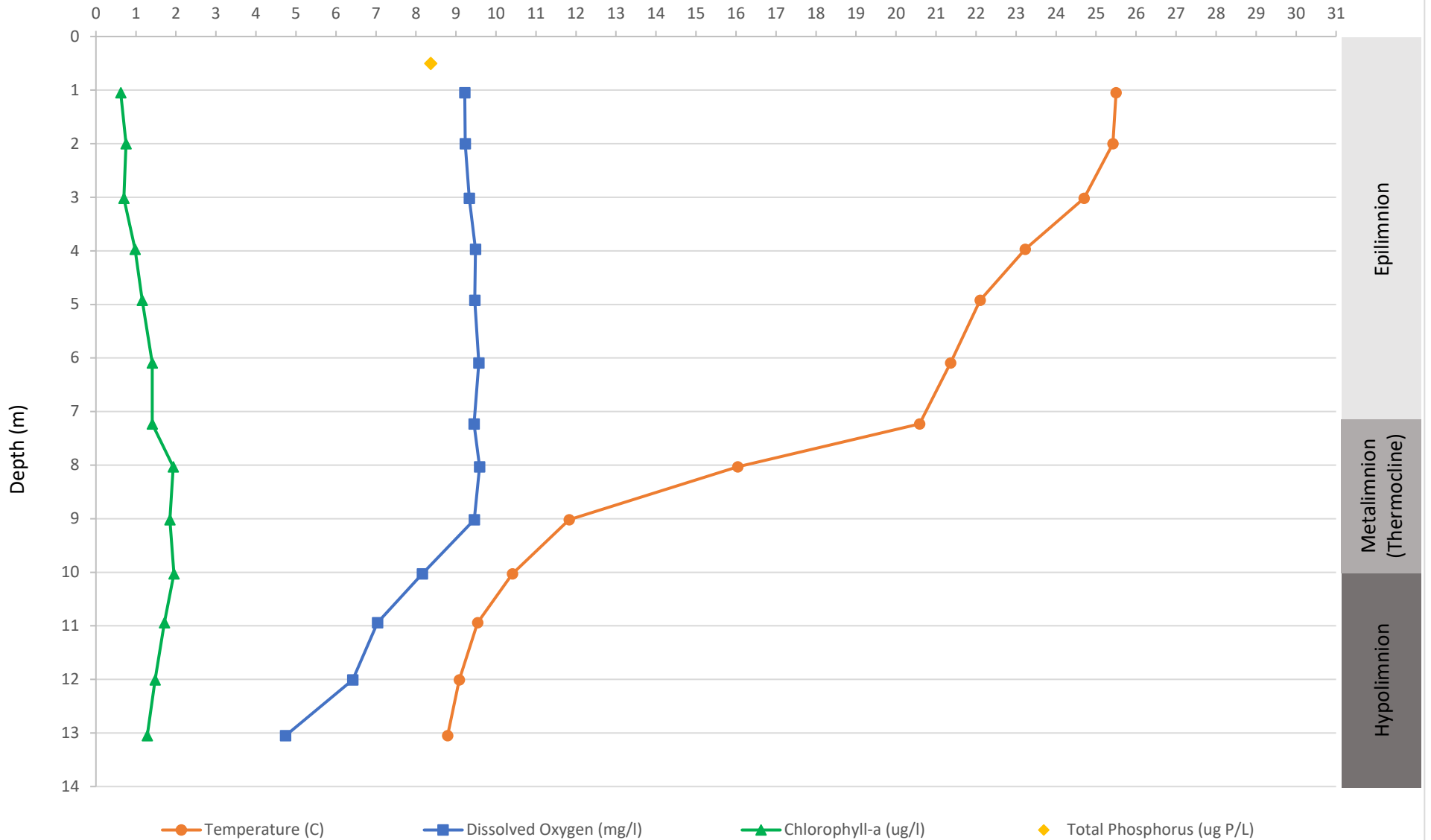
Lake Bomoseen Station 1 Temperature, Dissolved Oxygen, Chlorophyll-a and Total Phosphorus Vertical Profiles on 7/2/2018
