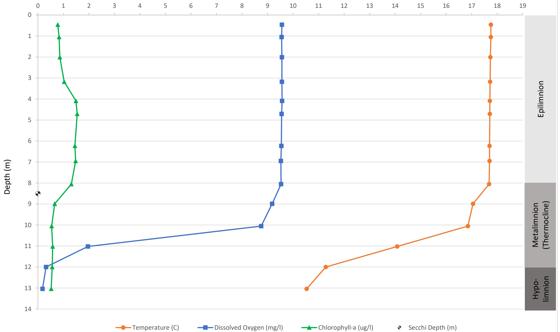
Lake Bomoseen Station 1 Temperature, Dissolved Oxygen and Chlorophyll-a Vertical Profiles on 10/12/2018
