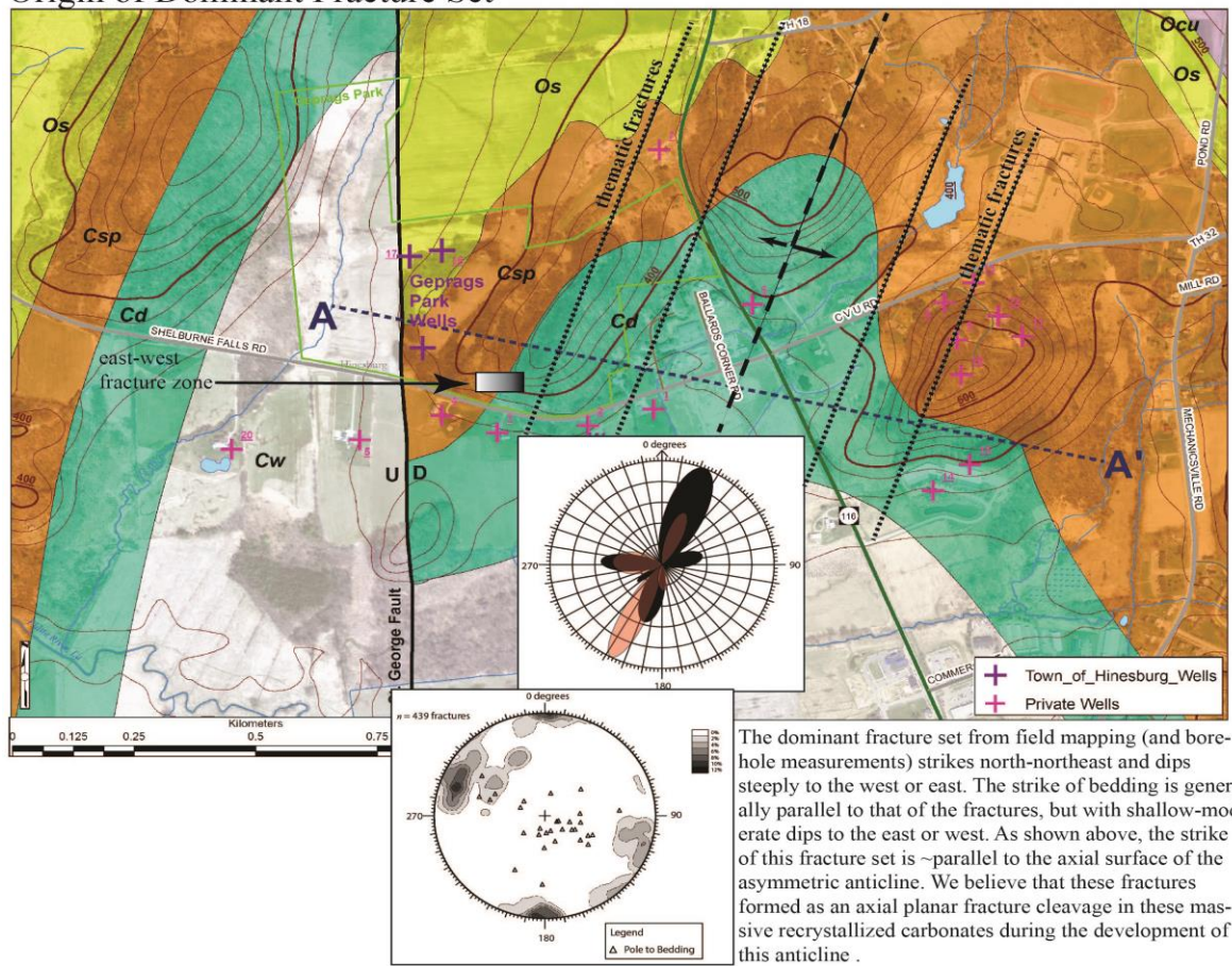
Figure 12. Rose diagram and equal area net for all structural data acquired in the field (black = fractures and red = bedding)(Salvini et al., 1999) overlaid on bedrock geologic map (modified from Kim et al. (2015). Map base modified from Ratcliffe et al. (2011). Note that the dominant fracture peak is axial planar to the fold in the Hinesburg Synclinorium.
