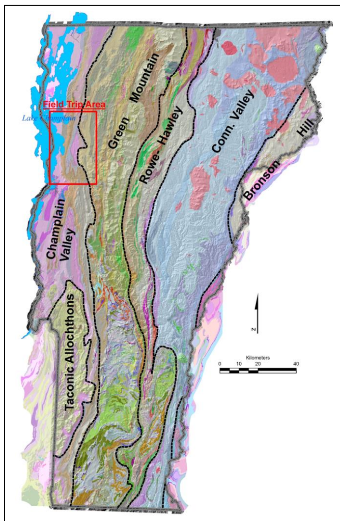
Figure 1. Tectonic belts in Vermont. Modified from Ratcliffe et al. (2011).
