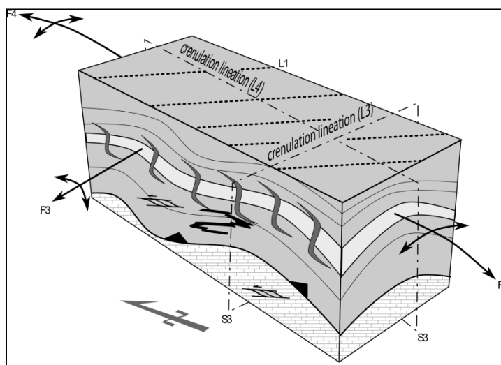
Figure 11. Block diagram showing the relative geometry of orthogonal fold sets that deform the Hinesburg Thrust surface and the mylonites at Mechanicsville, producing a dome and basin pattern. The two fold sets ( F_3 and F_4 ) are associated with two steeply dipping orthogonal cleavages.
