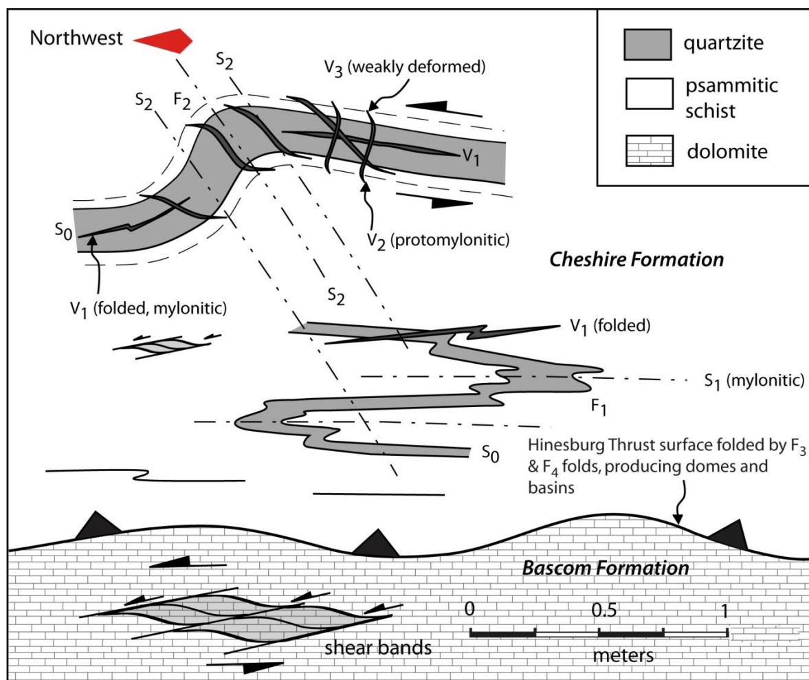
Figure 8. Sketch of structural relationships above and below the Hinesburg Thrust on vertical cliffs at Mechanicsville (Stop 5). Cliff face is oriented parallel to an L_1 quartz-mica mineral lineation.
