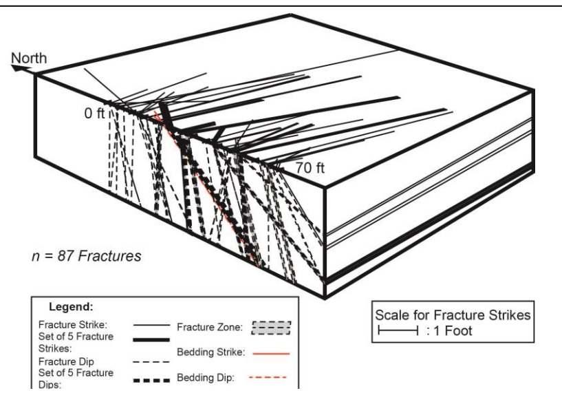
Figure 13. 3-D configuration of fractures at an outcrop in Geprags Park where east-west trending fractures are dominant (Chirigos, pers. comm., 2015)
