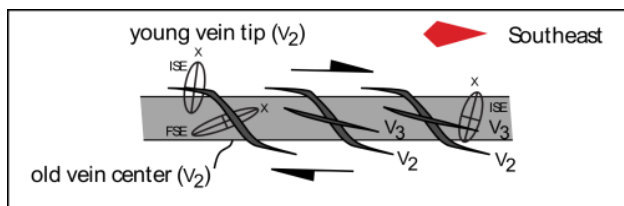
Figure 10. Cartoon showing an alternative model of progressive formation of vein sets during simple shear. This model requires the veins to continue to open during shearing. This model does not predict the correct orientation of V_3 veins or the top-to-the-NW sense of shear observed in the outcrop.
