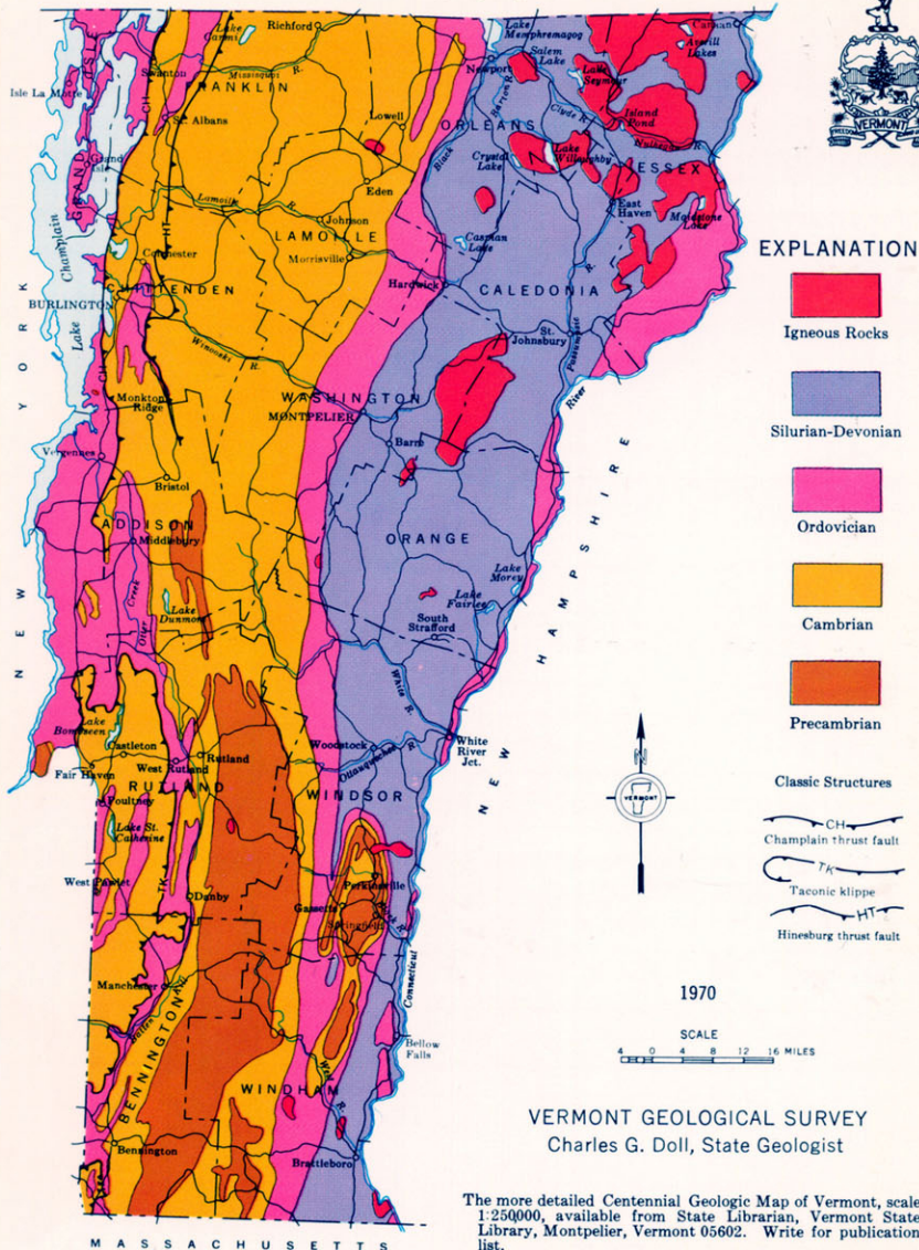
GENERALIZED GEOLOGIC MAP OF VERMONT
