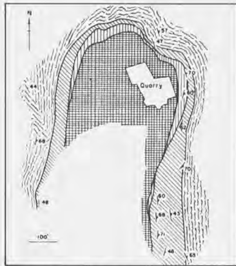
Metamorphosed ultramafic body \frac{1}{2} mile S40°W from North Hollow School, Rochester, Vermont
