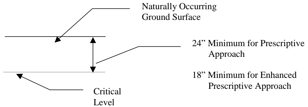
Figure 8.1 Critical Levels for Site Suitability Prescriptive and Enhanced Prescriptive Based Designs
