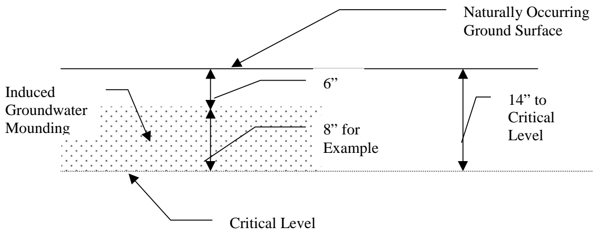
Figure 8.2 Critical Level for Site Suitability Performance Based Designs
