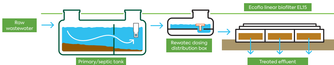
Figure 1.3.1 | Ecoflo linear EL15 biofilter system with gravity distribution
