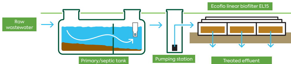
Figure 1.3.3 | Ecoflo linear EL15 biofilter system with low-pressure distribution
