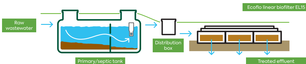
Figure 1.1 | Ecoflo linear EL15 biofilter system with gravity wastewater distribution
