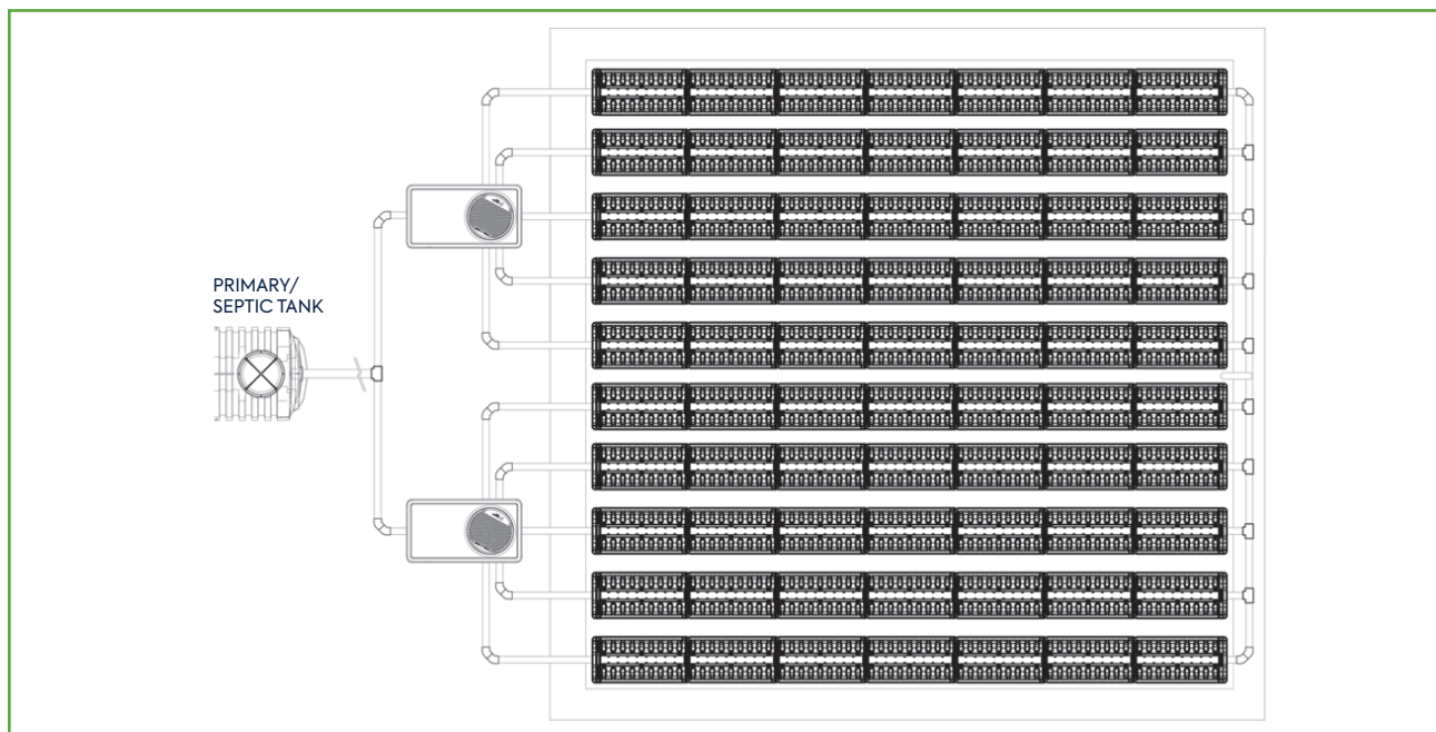
Figure 3.5.1.1 | Ten treatment lines installation fed by two Rewatec dosing distribution boxes
