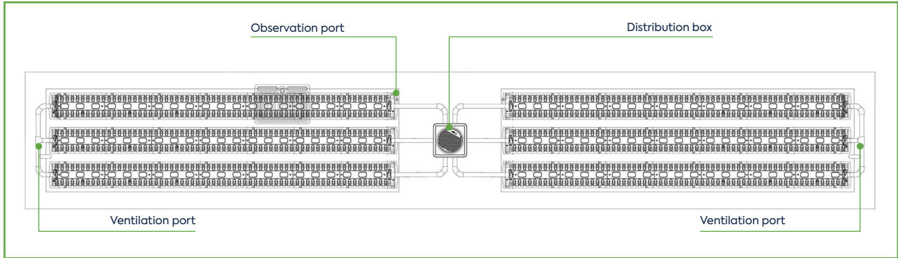
Figure 5.4.2 | Schematic of the ventilation of the Ecoflo linear biofilter EL15 with clusters of treatment modules
