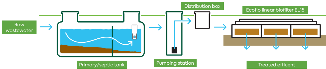
Figure 1.3.2 | Ecoflo linear EL15 biofilter system with pump-to-gravity distribution
